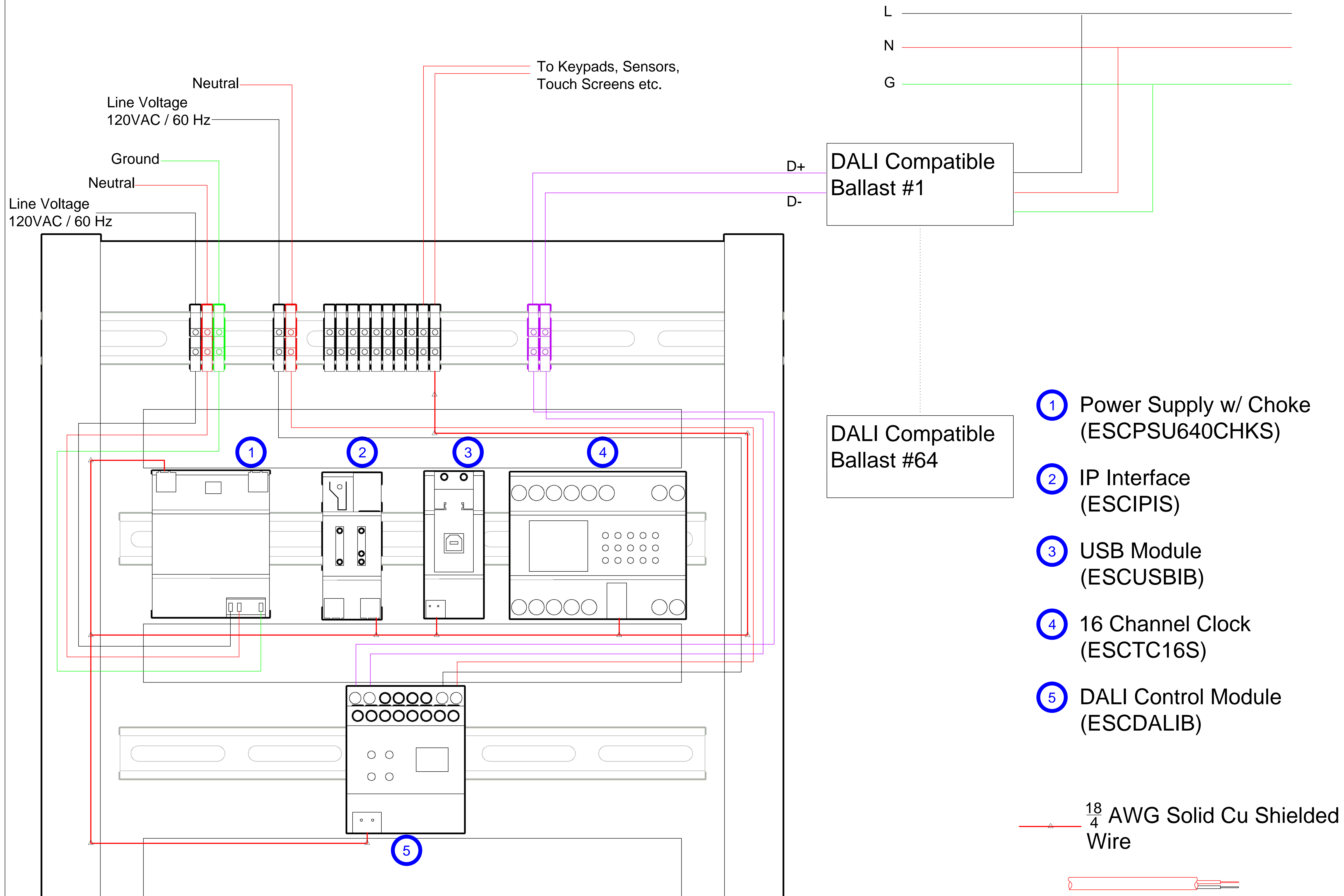
Lighting Control Panel Wiring Diagram
